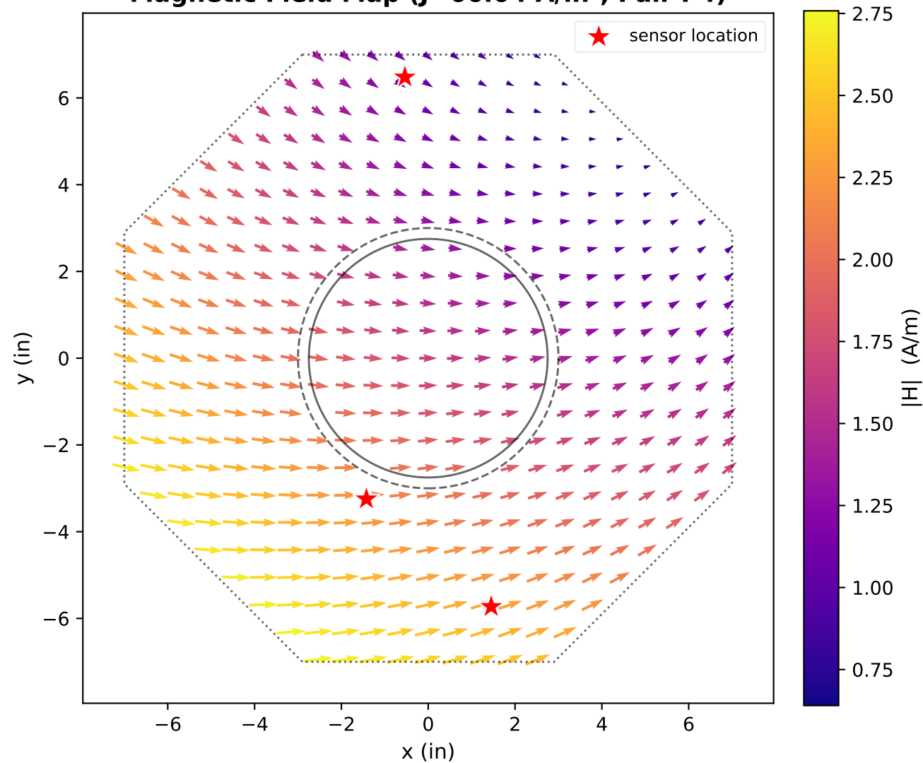
Magnetic Field Map ( J=66.04 A/in 2 , Pair P4)
